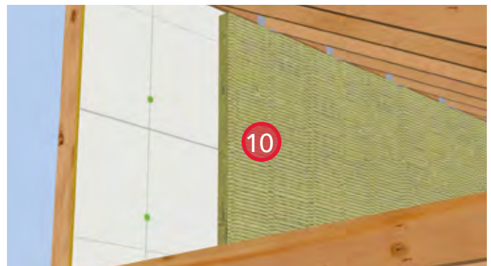
10. Install ROCKWOOL COMFORTBOARD™ 80 on the exterior of the wall between canopy ledger boards with recommended fasteners.
