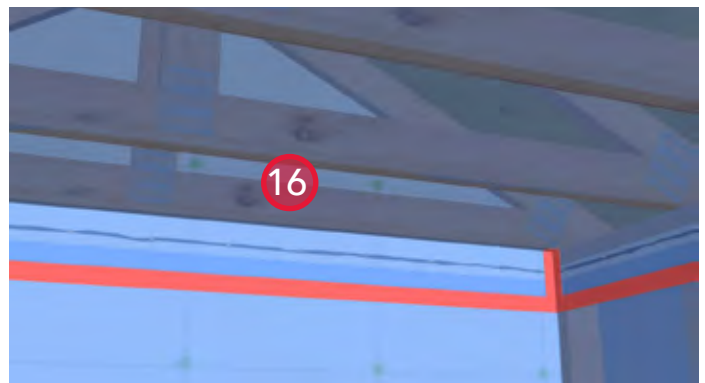
16. Install poly to the underside of the roof framing and fasten with staples at the sealant bead to complete the air seal. Seal the leading edge with sheathing tape.
