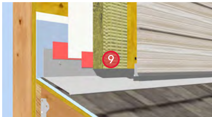
9. Install cladding and closure flashing.
