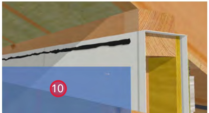
10. Install a bead of acoustical sealant on the sheathing membrane at the lower top plate to transition the air barrier from the wall to the ceiling.
