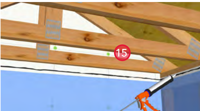
15. Install a bead of acoustical sealant along the sheathing membrane in line with the lower top plate of the exterior wall.
