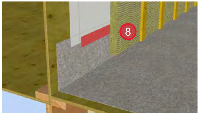
8. Install ROCKWOOL COMFORTBOARD™ 80 insulation and strapping to the exterior of the wall. Provide bugscreens at the top and bottom of the cladding.
